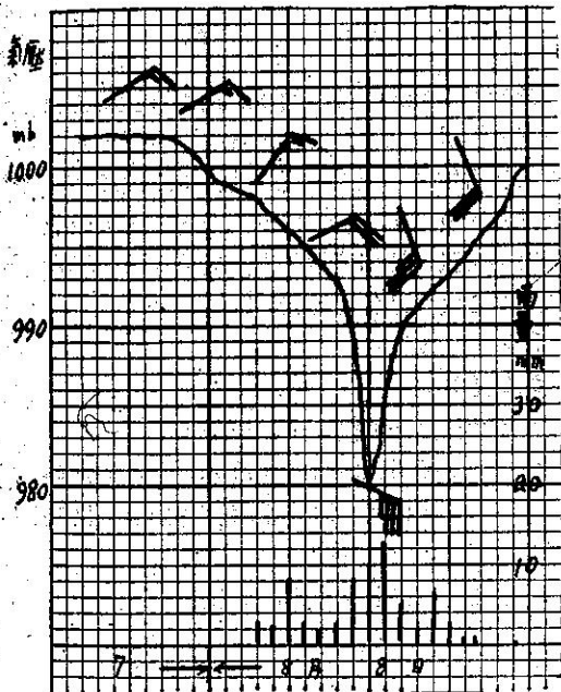
圖5. 貝蒂颱風過境期間彭佳嶼測得之氣壓，風 向風速及逐時雨量變化(全翹10m/s半翹5m/s) Fig 5. The sequence of pressure, wind direction & wind speed, and hourly rain- fall which was observed at Pengchayuan during Betty's passage. (whole bar- 10m/s, half bar-5m/s)
