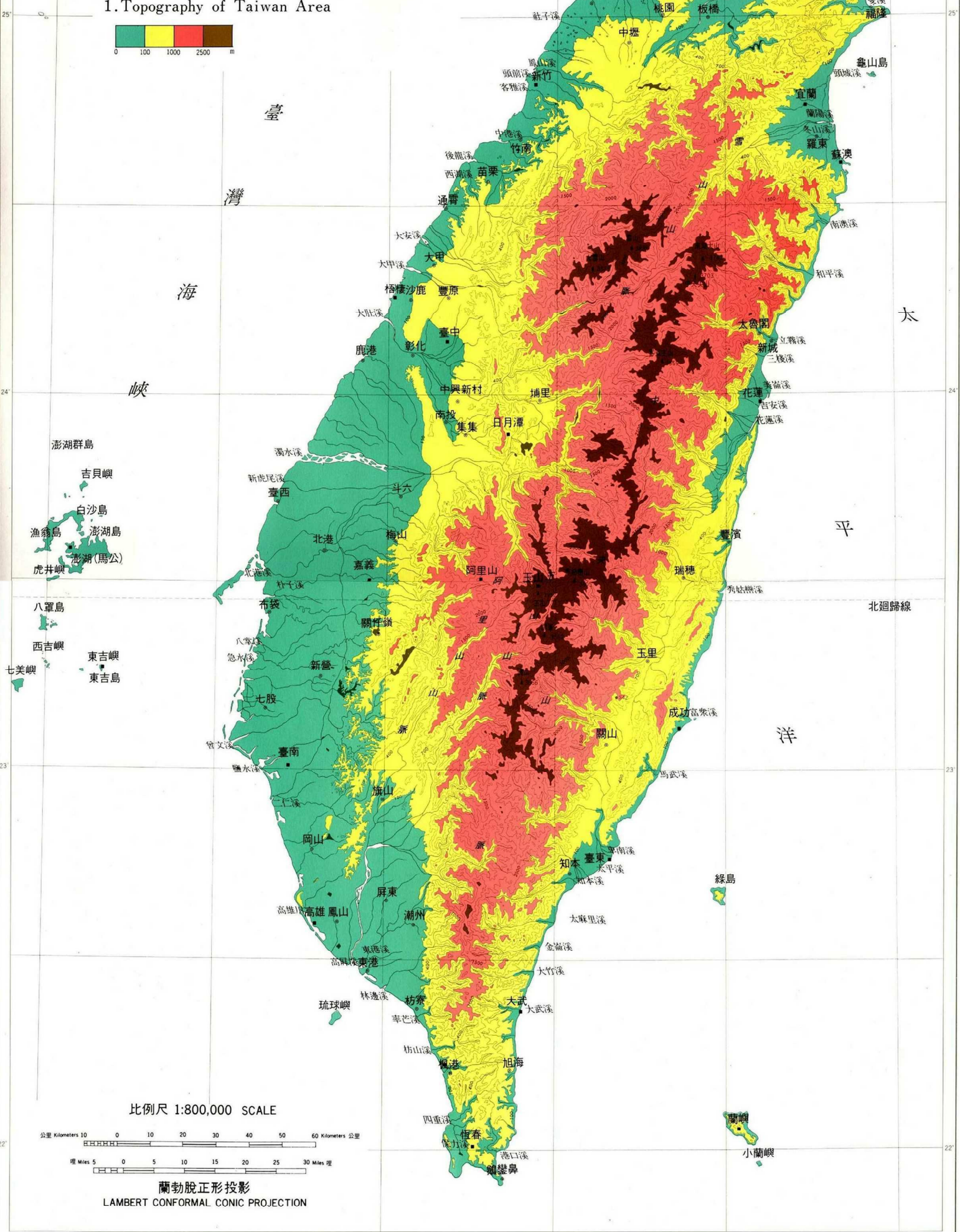
1. Topography of Taiwan Area
