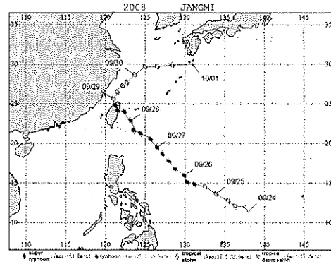
Fig. 1 Tracks of Typhoon Jangmi from best tracks of CWB. The symbol indicates the best track for every 6h and the label represents the date at 0000UTC.
