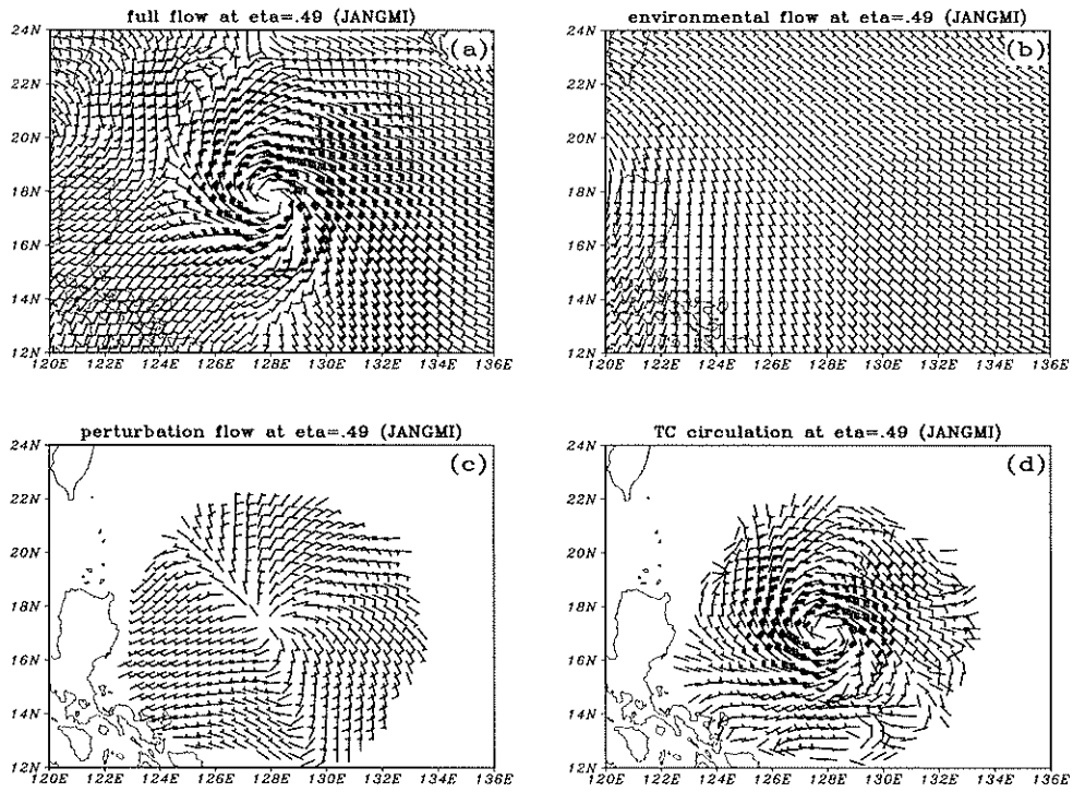
Fig. 2 The total atmosphere flow (Fig. 2a) decomposed into environmental flow (Fig. 2b), non-typhoon circulation (Fig. 2c), and typhoon circulation (fig.2d) with typhoon relocation procedure at 1200 UTC 26 September.
