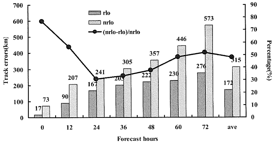
Fig. 6 The simulated typhoon track errors and the percentage differences of the track errors with (rlo) and without (nrlo) typhoon relocation procedure.
