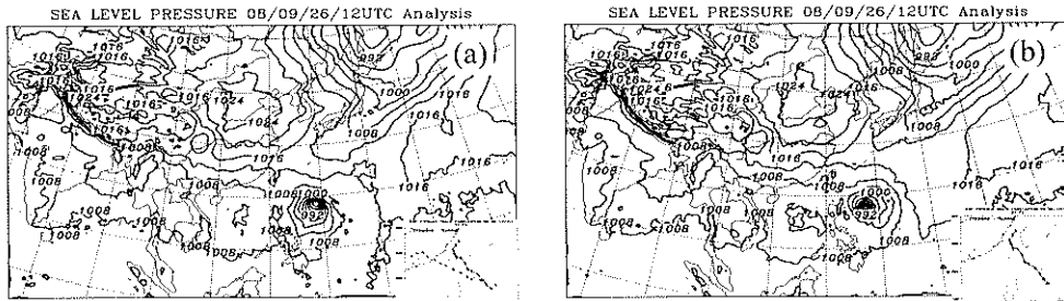
Fig. 7 The analysis fields of Sea Level Pressure without (a) and with (b) typhoon relocation procedure at 1200UTC 26 September. Tracks of Typhoon Jangmi from best tracks of CWB (black) and from the model 72 hours forecast at the same time (red and green for without and with typhoon relocation procedure, respectively) are also shown in the attached chart.
