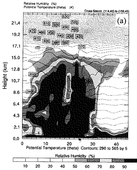
Fig. 8 Zonal cross section of potential temperature (with contour interval of 5K) and relative humidity (shaded for every 10%) cutting through typhoon center without (a) and with (b) typhoon relocation procedure.
