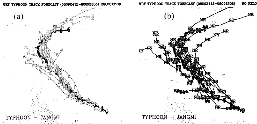
Fig. 5 Tracks of Typhoon Jangmi from best tracks of CWB (black) and with (a) and without (b) typhoon relocation procedure from 1200UTC 24 to 0600UTC 28 September. The typhoon symbol indicates the tracks for every 6 h.
