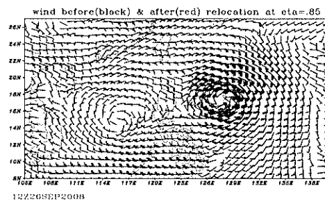
Fig. 4 Similar with Fig.3 except for the wind field distribution and the blue, red, black typhoon symbols represent typhoon center of observation, with and without typhoon relocation procedure, respectively.
