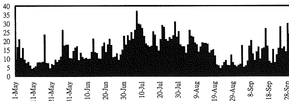
RCMs 200805_FCST_Tai_PCP_Anomaly
