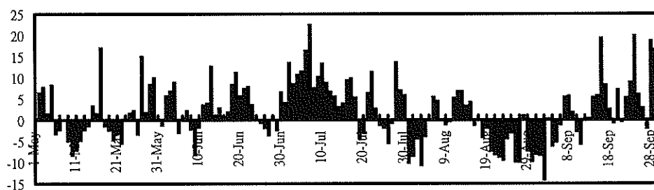
RCMs 200805_FCST_Tai_PCP
