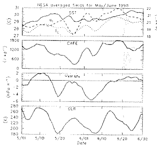
Fig. 10. Time series of SST (solid), surface air temperature T_0 (dotted), surface specific humidity q_0 (dashed), CAPE, vertical motion at 400 hPa, and OLR over the NESA for May and June 1998. Shaded times are outside the SCSMEX IOP.
