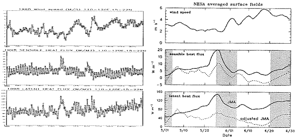
Fig. 11. Time series of wind speed and adjusted (dashed line) and unadjusted (solid line) JMA/GAME Reanalysis sensible and latent heat fluxes. Adjusted fluxes are based on measurements of bulk fluxes from Shiyan #3 (see text for explanation). Times when Shiyan #3 was off station are shaded.
