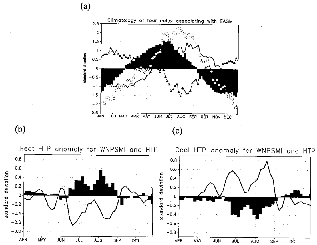
Figure 1. (a) Seasonal variation in four indexes: western North Pacific summer monsoon index (WNPSMI —, Wang et al. 2001), Tibetan Plateau heating (HTP ■, Hsu and Liu 2003), East Asia monsoon index (EAMI ○, Zhu et al. 2005) and Asian continental pattern index (ACPI ▲, Krishnan and Sugi 2001). The unit has been normalized. (b) Composite of positive HTP anomaly (heating anomaly, 1991, 1995, 1998 and 1999) in WNPSMI and HTP. (c) The same as (b) but for cooling anomaly years (1984, 1986, 1990, 1994, 1997 and 2001).
