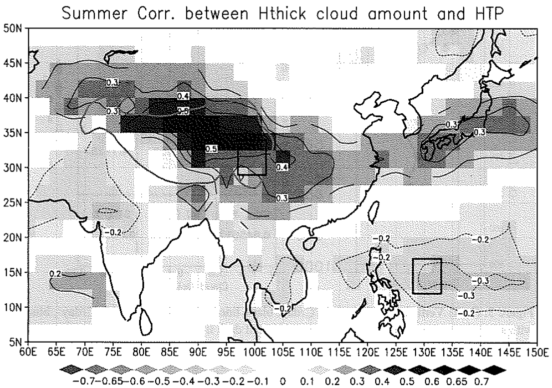
Figure 2. Pentad correlation coefficient in summer between (a) High-thick cloud amount and WNPSMI and (b) High-thick cloud amount and HTP.
