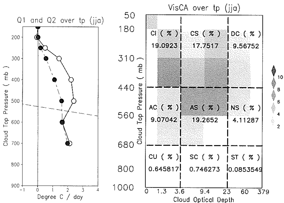
Figure 3. (Left) Vertical profile of Q1 ( ^{\circ}\text{C}/\text{day} , black line with symbol \circ ), Q2 ( ^{\circ}\text{C}/\text{day} , blue line with symbol \bullet ) and atmospheric temperature ( ^{\circ}\text{C} , red dash line). (Right) Vertical profile of visible cloud amount (%), based on the classification in ISCCP). The data is average in summer in the area-mean of (a) TWNP ( 128^{\circ}\text{E}\sim 133^{\circ}\text{E} , 12^{\circ}\text{N}\sim 17^{\circ}\text{N} ) and (b) TP ( 97^{\circ}\text{E}\sim 102^{\circ}\text{E} , 29^{\circ}\text{N}\sim 34^{\circ}\text{N} ).
