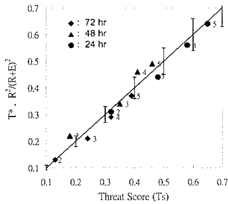
FIG. 2. Plot of the estimate threat score and of the threat score in 24-/48-/72-h for the domains with radii of 200, 300, 400 and 500 km circled the point of 23.5°N and 121°E. The numbers on the right side of symbols are the radii in the unit of hector- kilometer.
