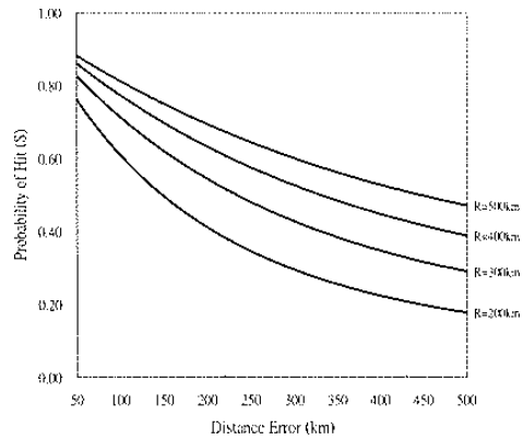
FIG. 3. Plot of probability of hits ( S^* ) as the function of mean distance error for the domains with radii of 200, 300, 400 and 500 km circled the point of 23.5°N and 121°E.
