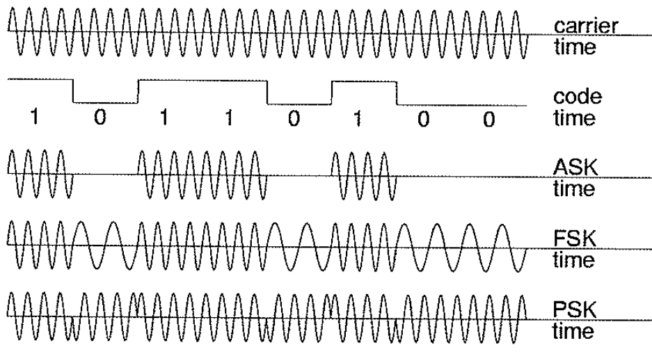
Figure 1. GPS signal structure. GPS use PSK form to transport signal.
