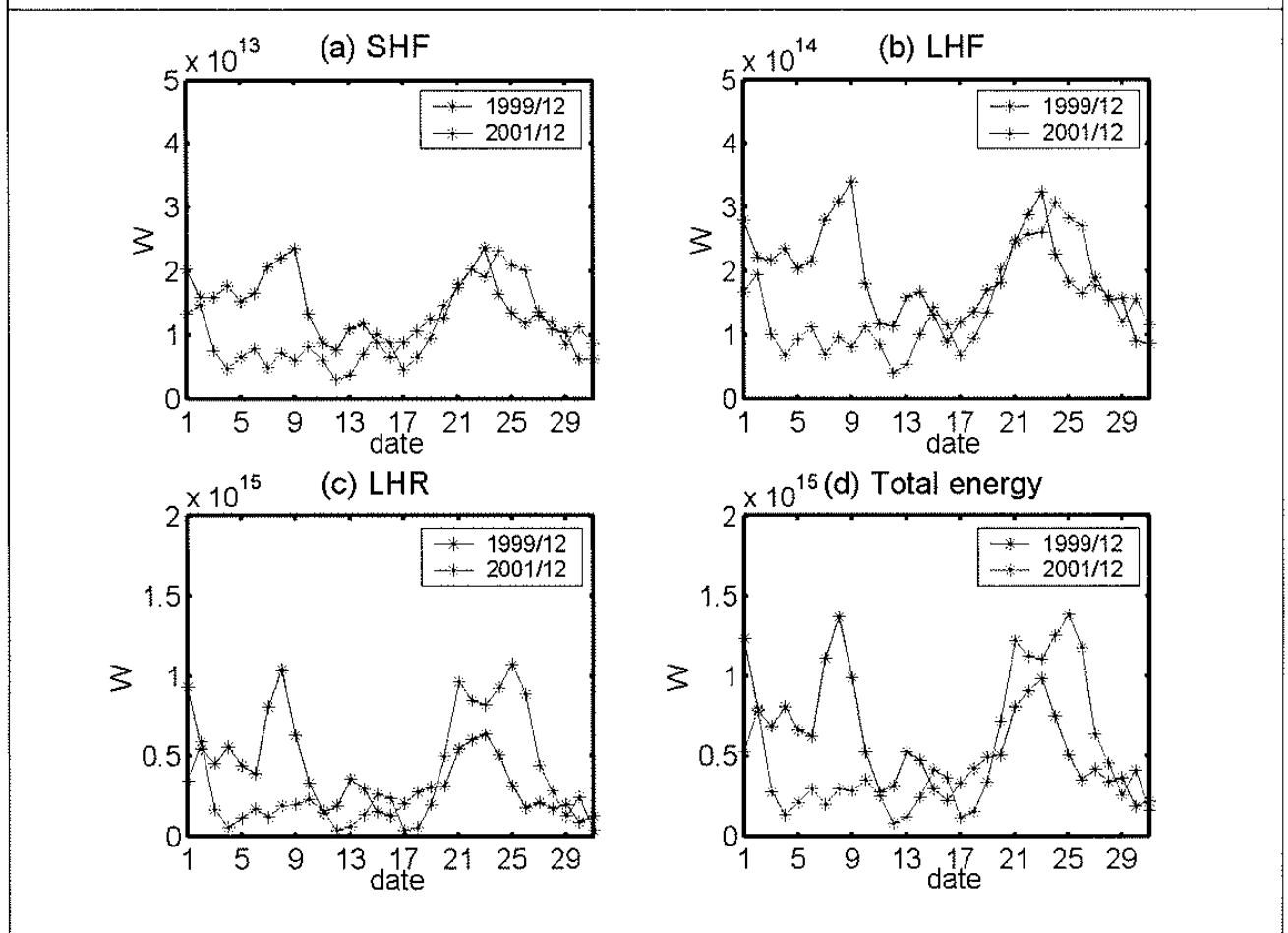
Fig. 1. Comparisons of (a) SHF, (B) LHF, (c) LHR and (d) Total energy in December of 1999 and 2001.
