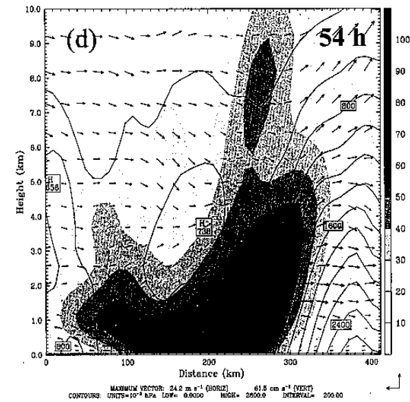
Fig. 9. Vertical cross section along the moving direction of Xangsane, showing pressure perturbation (solid, every 200 mini hPa), wind vectors (relative to the moving storm) and relative vorticity (shaded 10^{-5} \text{ s}^{-1} ) for 51h - 54h simulation.
