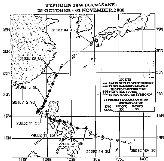
Fig. 1. The best track of Xangsane (2000). Symbols show 6-hourly positions (adapted from JTWC Annual Tropical Cyclone Report).
