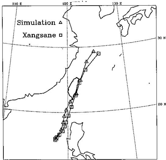
Fig. 4. Observed (labeled on the right side) and model simulated (labeled on the left side) tracks from 0000 UTC 30 October to 1200 UTC 1 November 2000.
