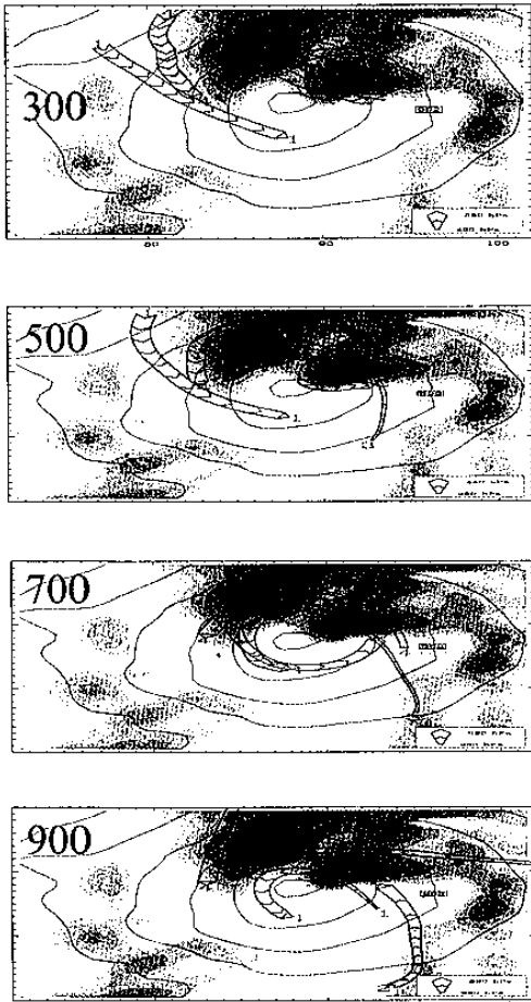
Fig. 8. Five-hour (49 h to 54 h) backward trajectories from 0600 UTC 1 November 2000 relative to the moving storm center for air parcels located at 90 km to the south (1), east (2), north (3) and west (4) of the storm center at 300 hPa 500 hPa 700 hPa and 900 hPa (from top to bottom)
