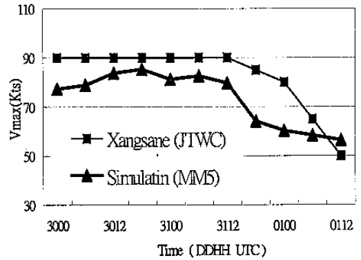
Fig.5. Observed and Model-simulated intensity of Xangsane from 0000 UTC 30 October to 1200 UTC 1 November 2000.
