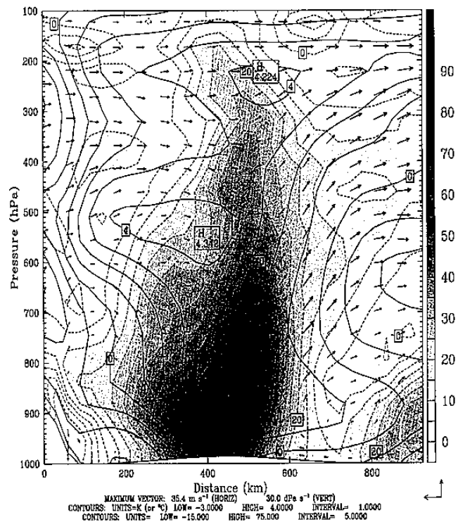
Fig. 7. Vertical cross section along the moving direction of Xangsane showing temperature anomaly (solid every 1 k), wind vectors along the moving direction and relative vorticity (shaded) for (a) 0600 UTC 31 October (30h), and (b) 0600 UTC 1 November 2000 (54h).
