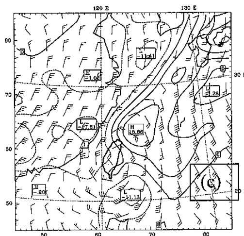
Fig. 3. (a) Sea surface pressure (every 4 hPa), and surface wind barbs (full barb = 10 kt), (b) 200 hPa wind barbs and total wind speed (shaded) and (c) 850hPa temperature advection (every 6 °C s -1 ) at 0000 UTC 1 Nov.
