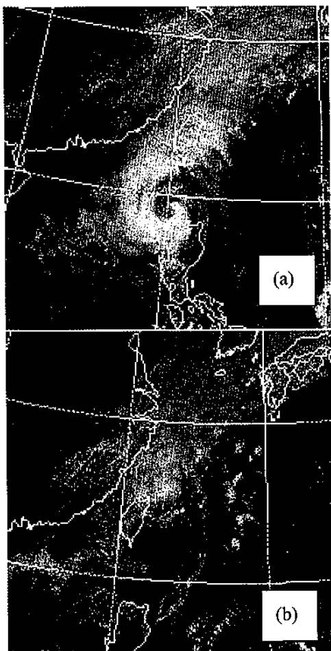
Fig. 2. GMS5 visible satellite image of Xangsane at (a) 0400 UTC (1200 LST) 31 October, and (b) 0400 UTC 1 November 2000.
