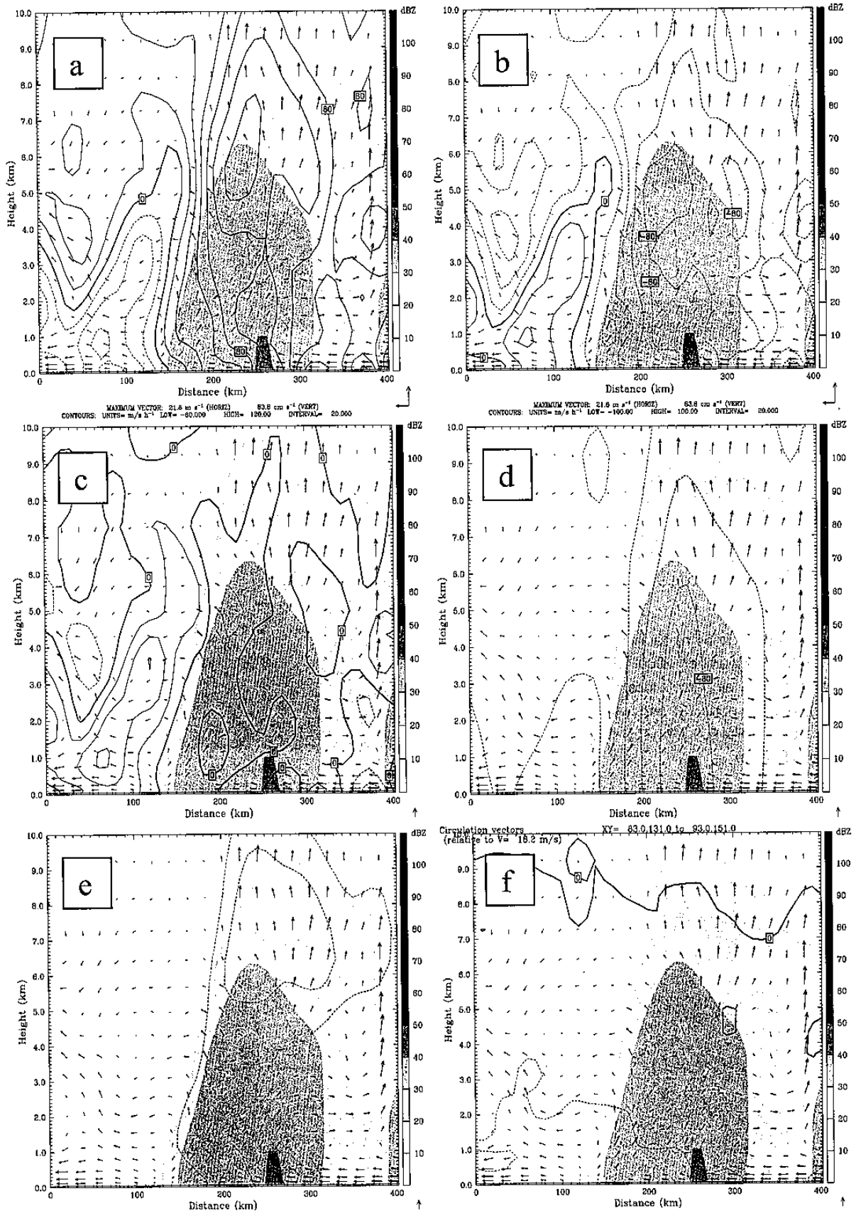
Fig. 10. As in Fig. 9 but for vertical momentum budget: (a) the perturbation PGF, (b) the buoyancy force (BU), (c) the thermal buoyancy force (BUTV), (d) the dynamic buoyancy force (BUD), (e) the water loading (WL), (f) summation (PGF + BU + WL). Dashed curves are negative values (every 20 \text{ ms}^{-1}\text{h}^{-1} ). The shading shows the reflectivity (in dBZ).
